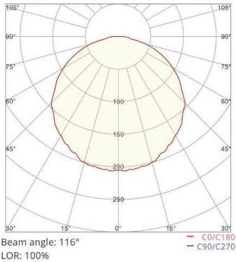
Polar plot
