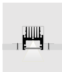
Incasso Recessed
